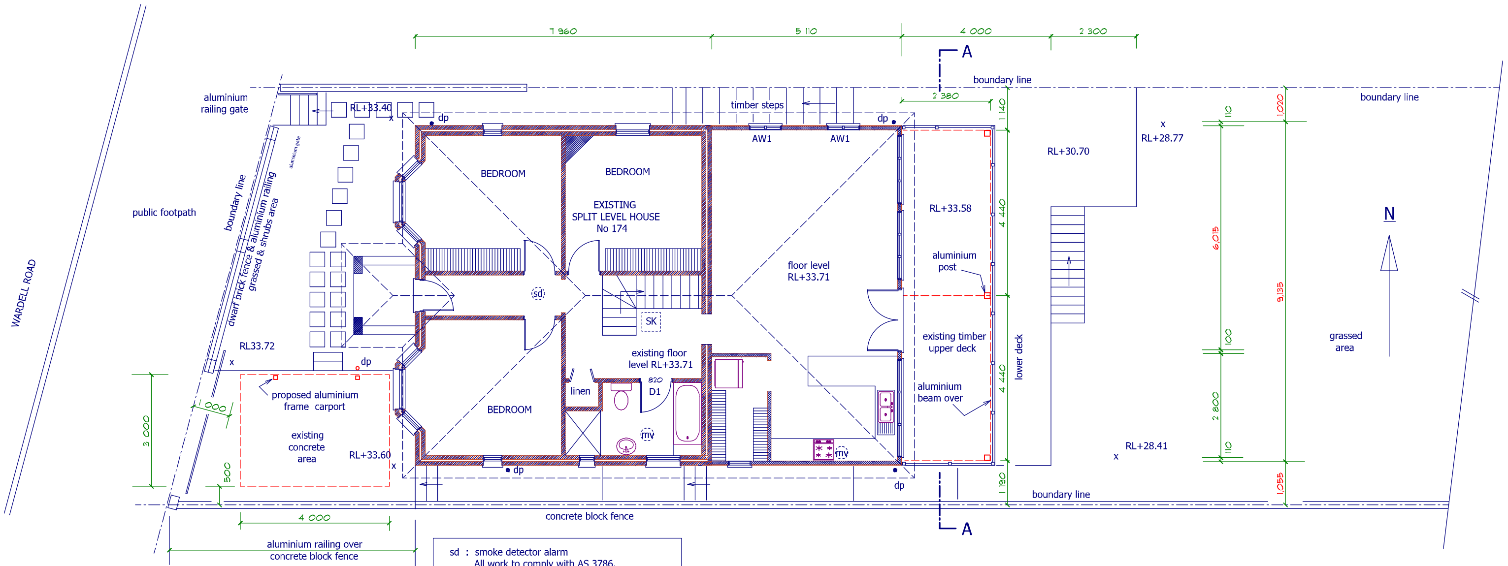
MAIN LEVEL FLOOR PLAN
