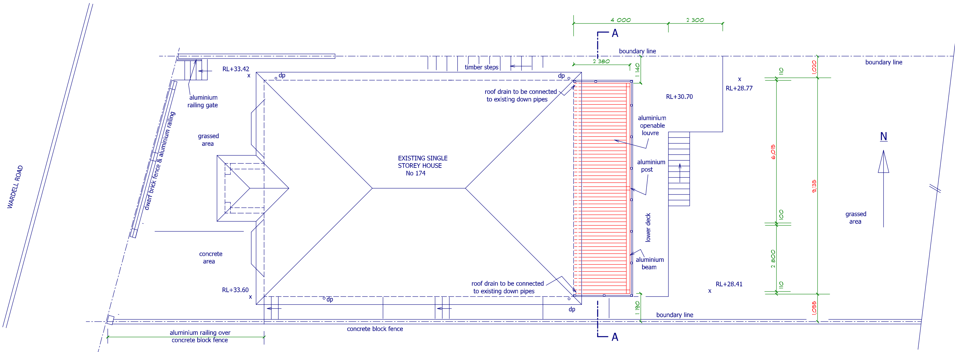
ROOF PLAN
